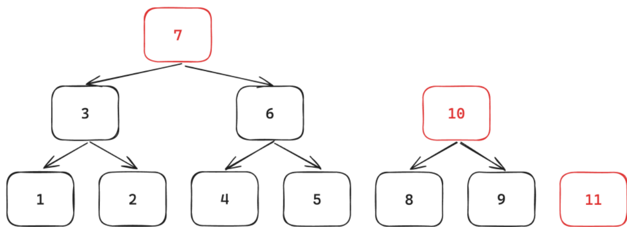
Figure 2: Merkle mountain rage (roots are red)
